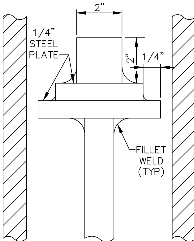
EXTENSION DETAIL
