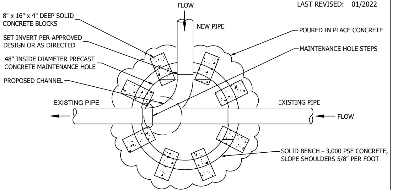
PLAN NTS
