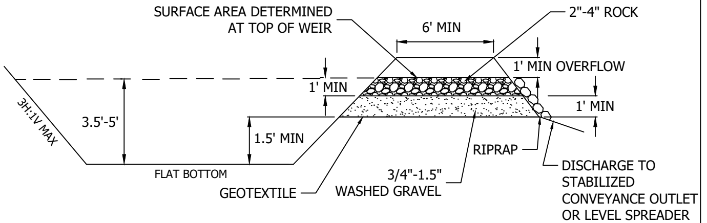
CROSS-SECTION
