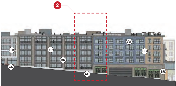
1 EAST ELEVATION
