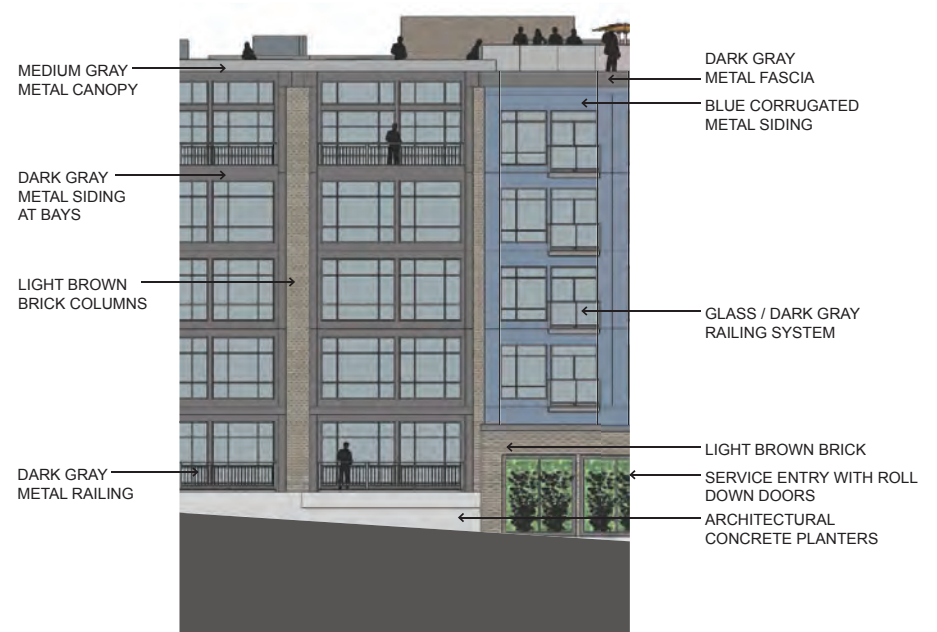
2 ENLARGED EAST FACADE DETAILING
