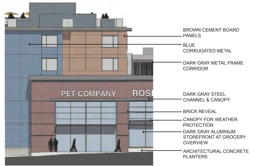
2 ENLARGED SOUTH FACADE DETAILING
