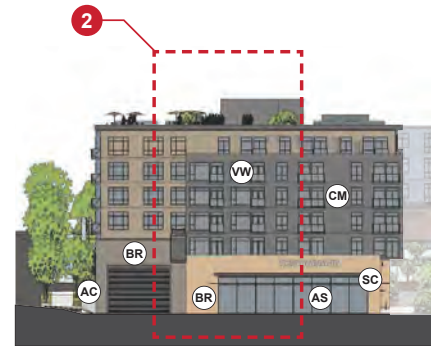
1 NORTH ELEVATION SCALE: 1"=50'-0" @ 11x17
