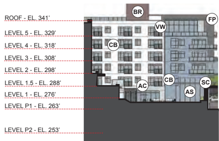
4 COURT EAST ELEVATION
