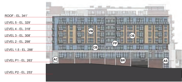
2 NORTH ELEVATION
