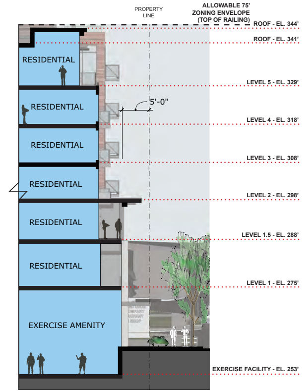
A WALL SECTION
