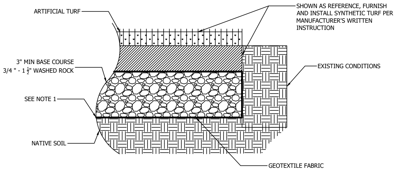
ARTIFICIAL TURF SECTION
