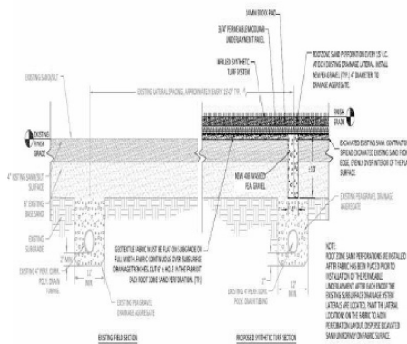
C OVERLAY NOT TO SCALE
