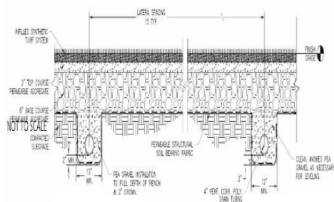
A TRADITIONAL FULL-SECTION CRSTWOODS NOTE: REPLACE EXISTING DRAINAGE AGGREGATE
