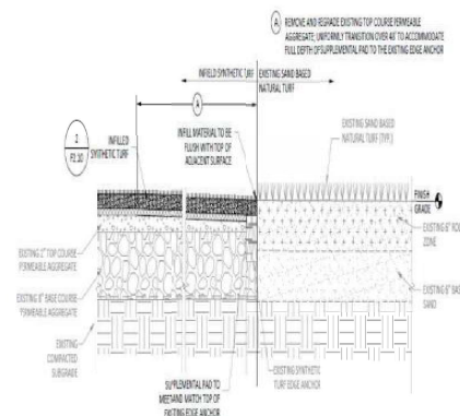
G EDGE ANCHOR @ GRASS TRANSITION NOT TO SCALE
