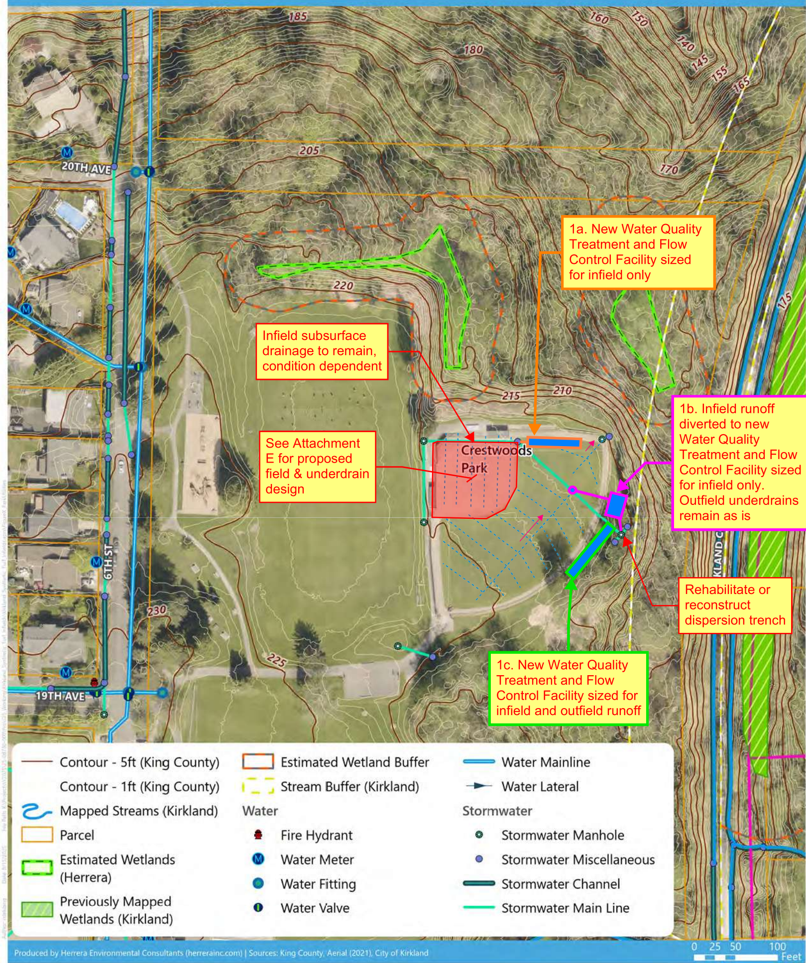
Figure D2. Crestwoods Park - Stormwater Option 1.
