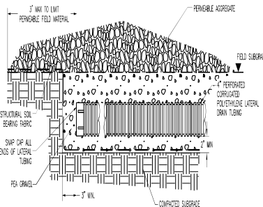
D TRENCHED SUBSURFACE DRAINAGE NOT TO SCALE
