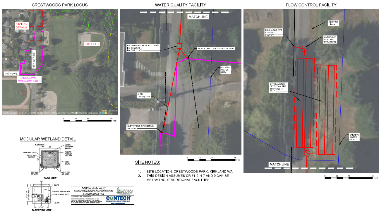
Figure G2. Crestwoods Park: Area-Swapped Flow Control
