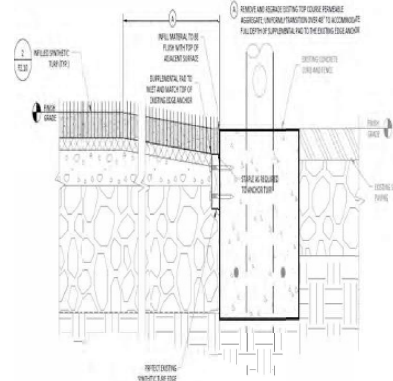
F CONTAINMENT CURB & EDGE ANCHOR NOT TO SCALE CRESTWOODS NOTE: CURB IS EXISTING
