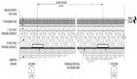
B FULL-SECTION w/ FLAT DRAINS NOT TO SCALE
