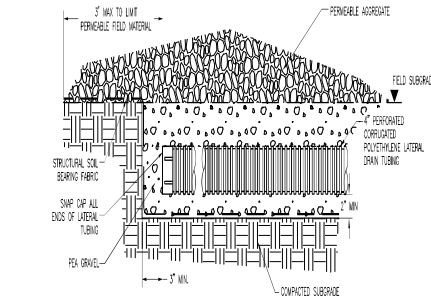
D TRENCHED SUBSURFACE DRAINAGE NOT TO SCALE
