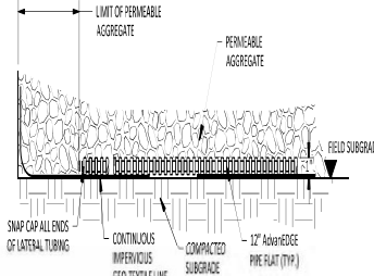
E FLAT / PANEL DRAIN NOT TO SCALE
