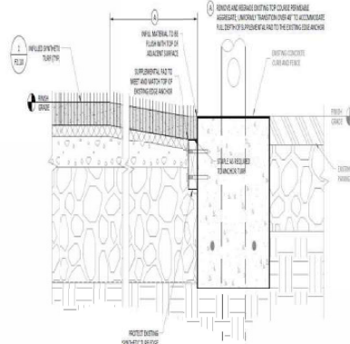
F CONTAINMENT CURB & EDGE ANCHOR CRSTWOODS NOTE: CURB IS EXISTING NOT TO SCALE
