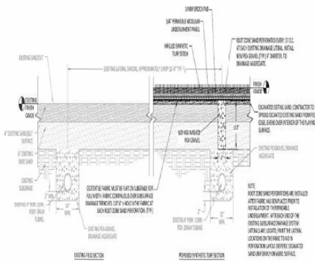
C OVERLAY NOT TO SCALE
