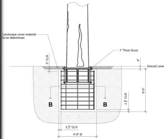
Pillar Weldment Detail Not to Scale Supplied by Cobalt Designworks
