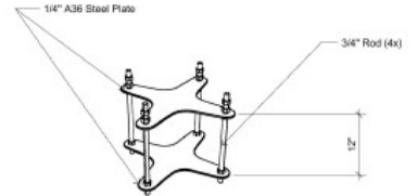
Cocoon Weldment Detail Not to Scale Supplied by Cobalt Designworks
