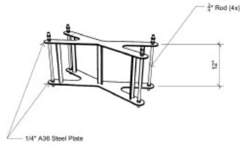
Pillar Weldment Detail Not to Scale Supplied by Cobalt Designworks
