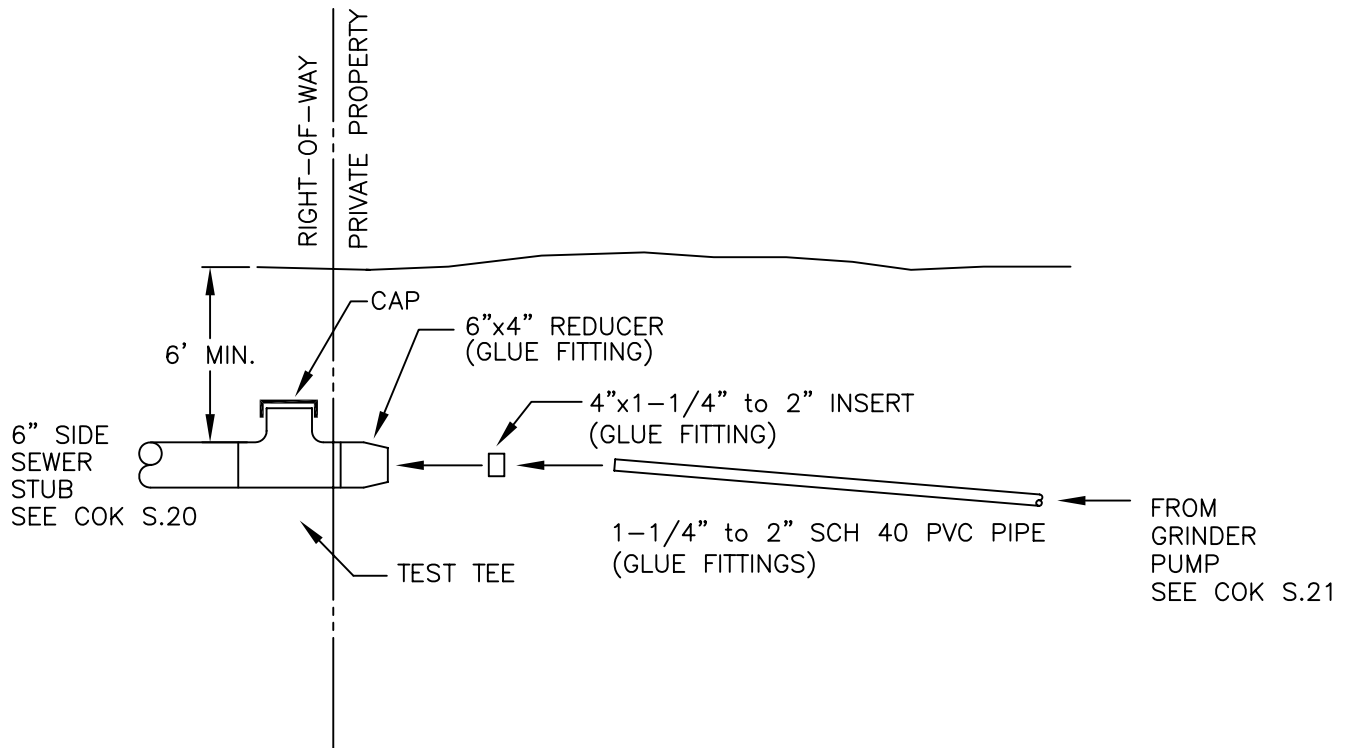
SECTION
