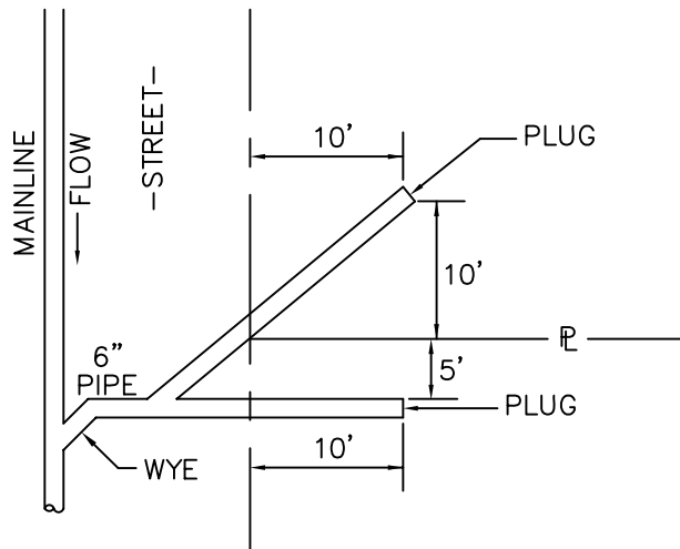
DOUBLE SERVICE
