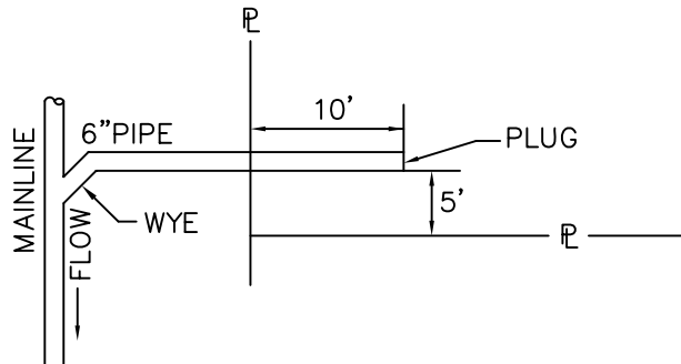
SINGLE SERVICE
