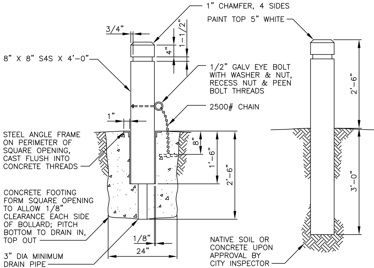
REMOVABLE BOLLARD
