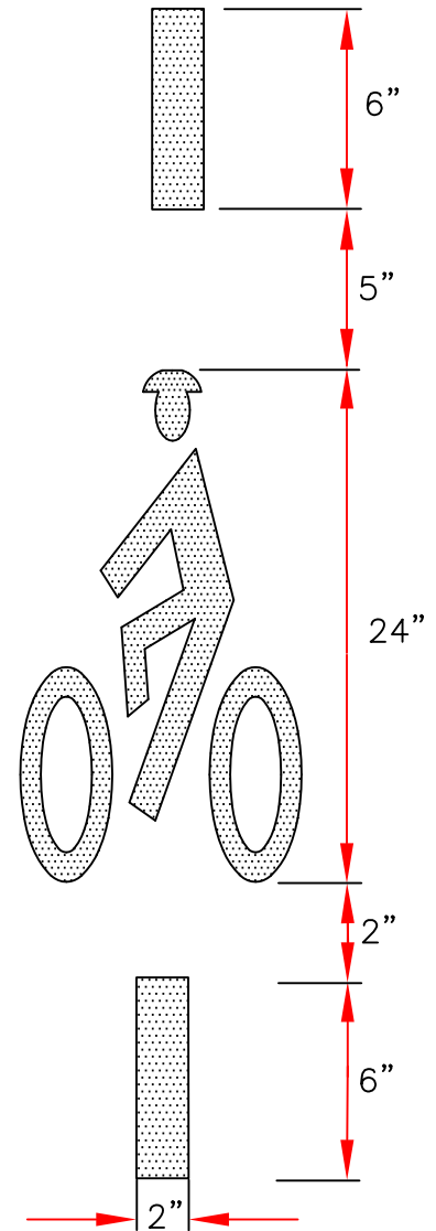
BICYCLE DETECTION MARKING DETAIL
