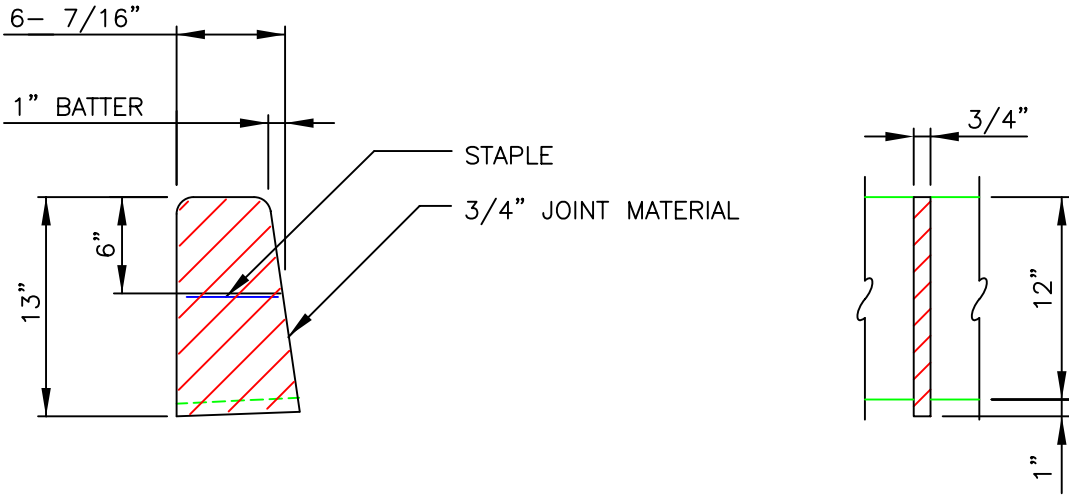
JOINT DETAIL
