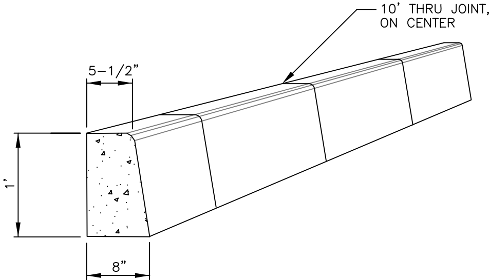
TYPICAL SECTION FOR VERTICAL CURB
