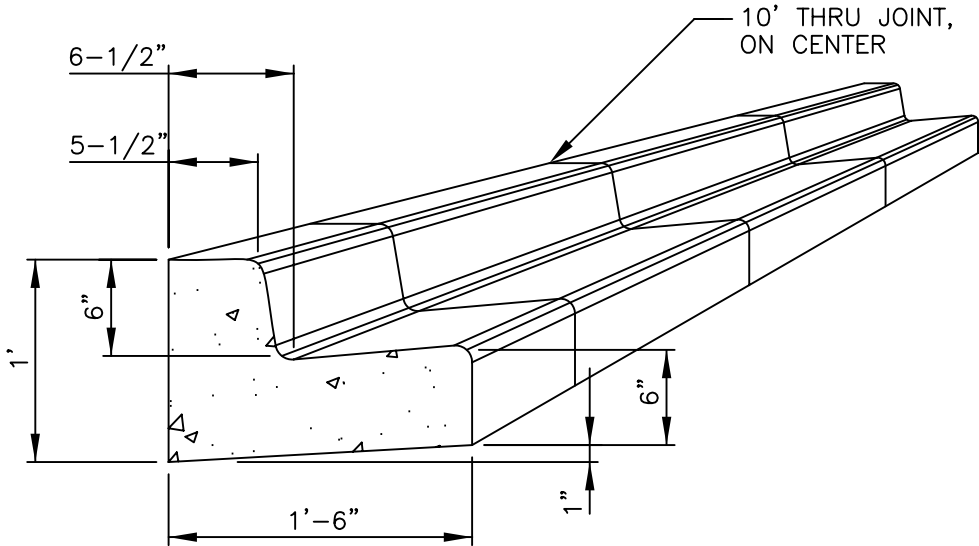
TYPICAL SECTION FOR CURB & GUTTER, TYPE A
