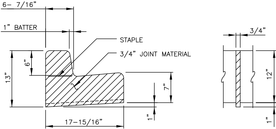
JOINT DETAIL
