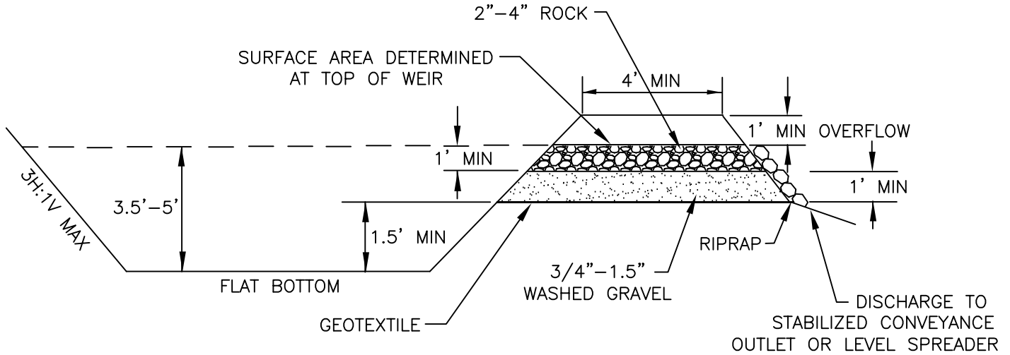
CROSS-SECTION
