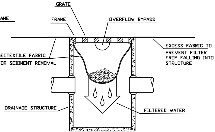
STORM DRAIN PROTECTION INSERT SECTION A-A NTS
